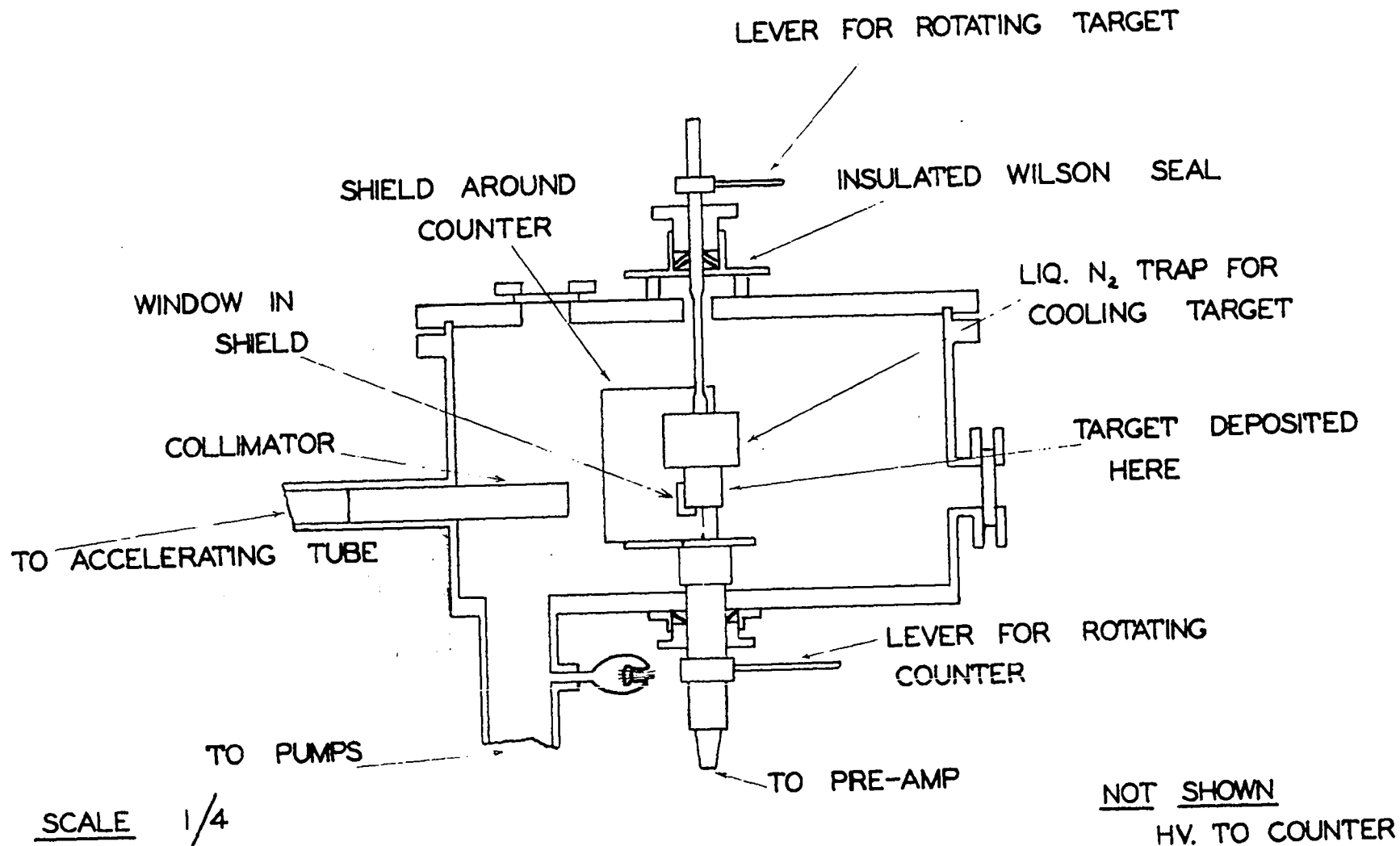
VACUUM TANK (SECTIONAL VIEW)
